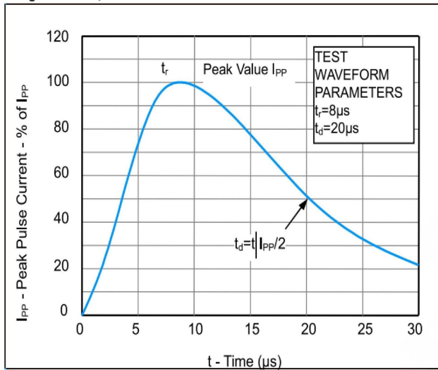
Fig1. 8/20 \mu\text{s} Pulse Waveform
