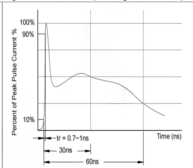
Fig2. ESD Pulse Waveform (according to IEC 61000-4-2)
