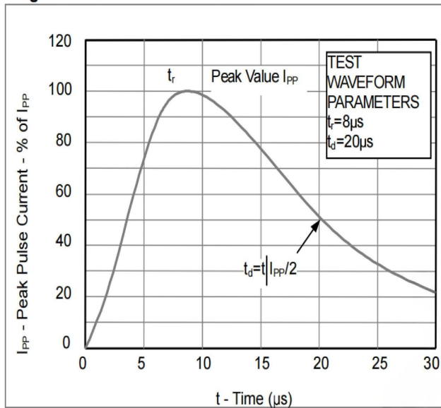
Fig1. 8/20 \mu s Pulse Waveform
