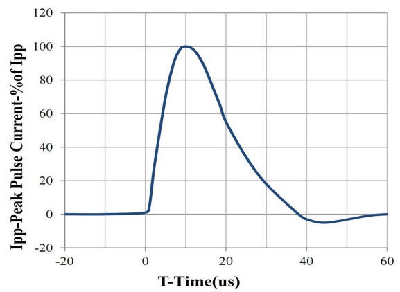
8 X 20us Pulse Waveform
