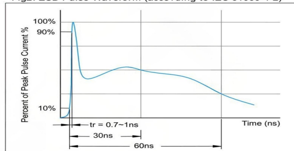
Fig2. ESD Pulse Waveform (according to IEC 61000-4-2)
