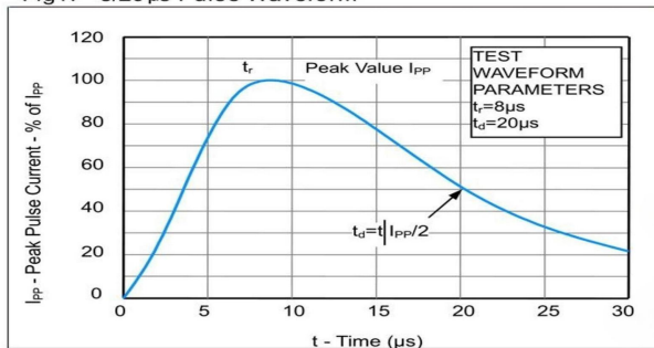
Fig1. 8/20μs Pulse Waveform
