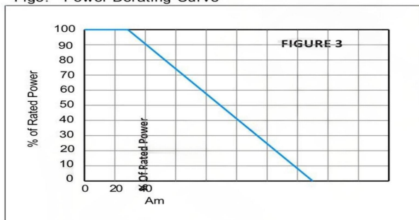
Fig3. Power Derating Curve
