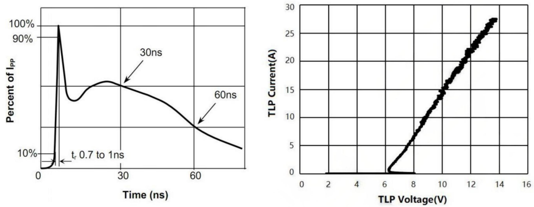
Fig.1 Pulse Waveform-ESD (IEC61000-4-2)
