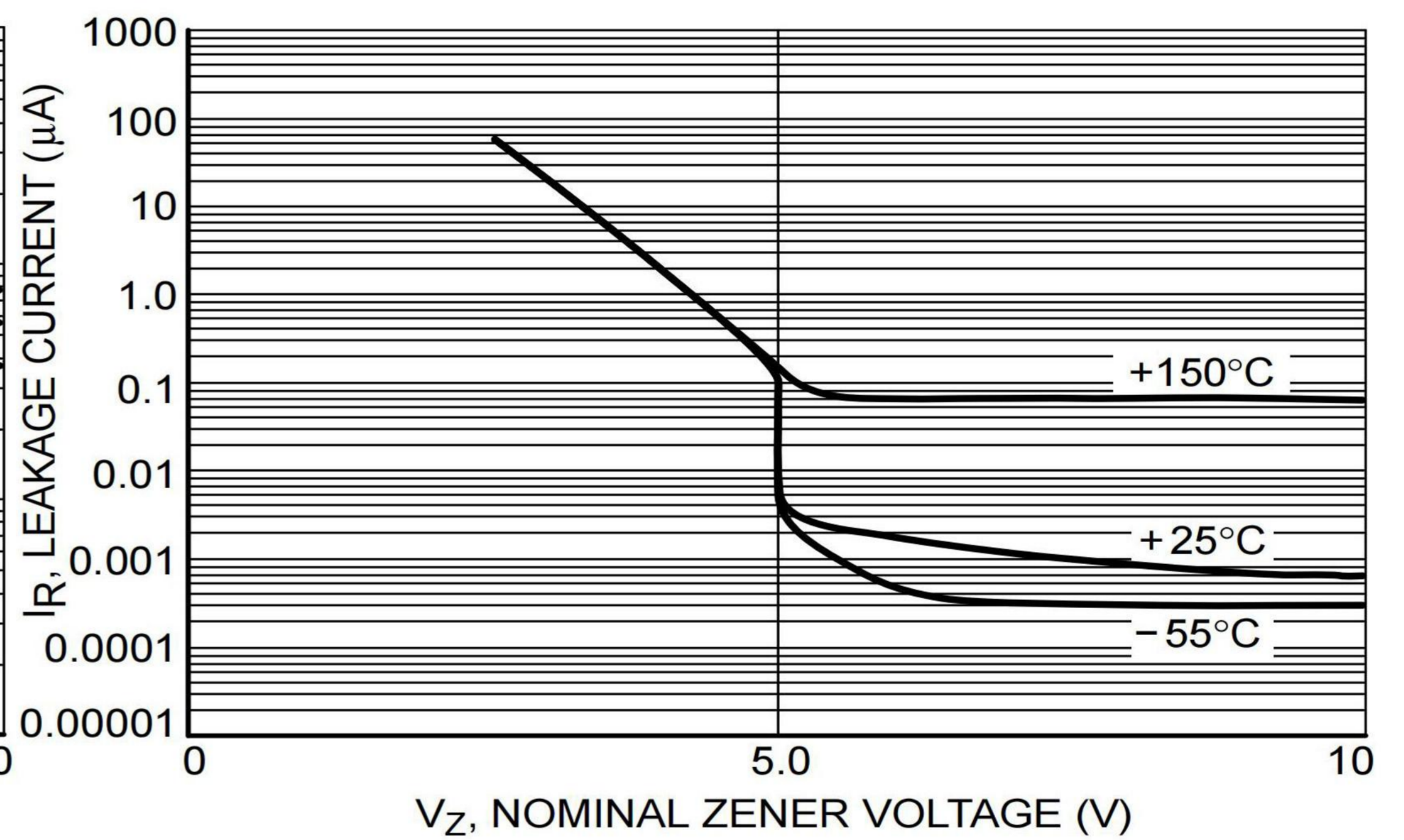
Figure 4. Typical Leakage Current
