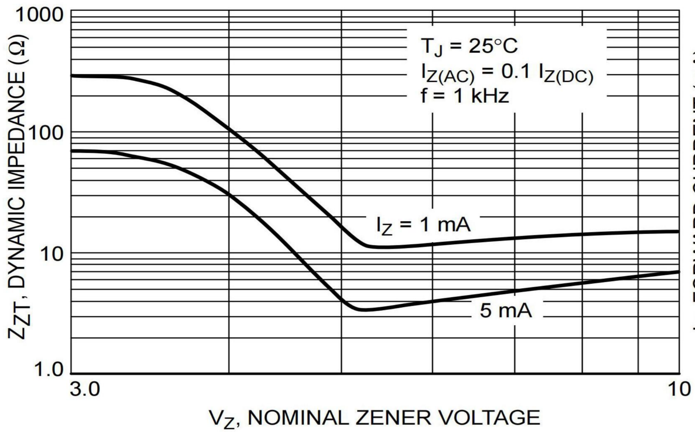
Figure 1. Effect of Zener Voltage on Zener Impedance
