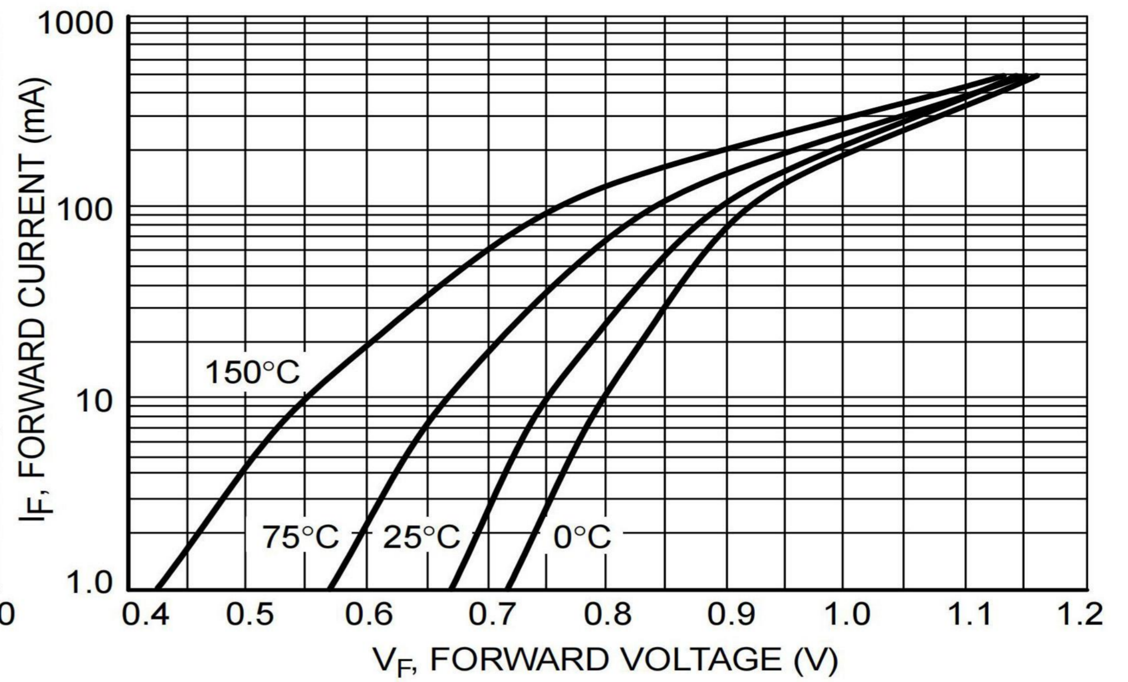
Figure 2. Typical Forward Voltage
