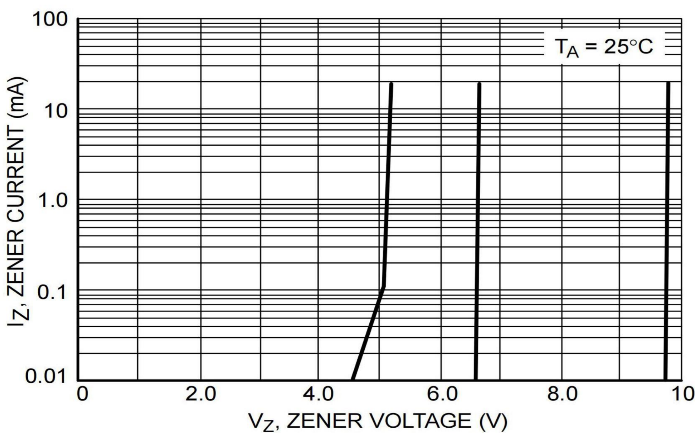
Figure 5. Zener Voltage versus Zener Current (V Z Up to 9 V)
