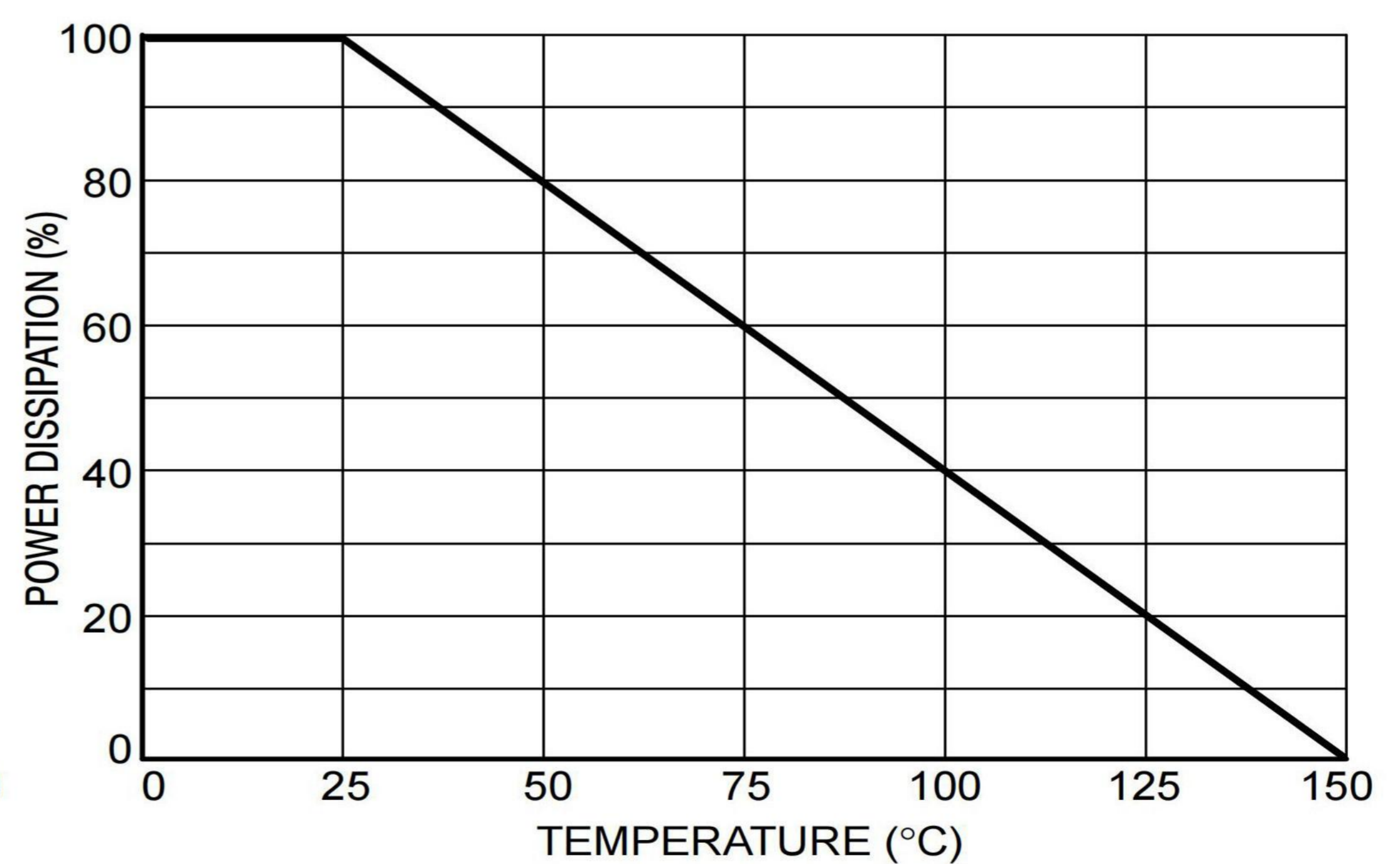
Figure 6. Steady State Power Derating
