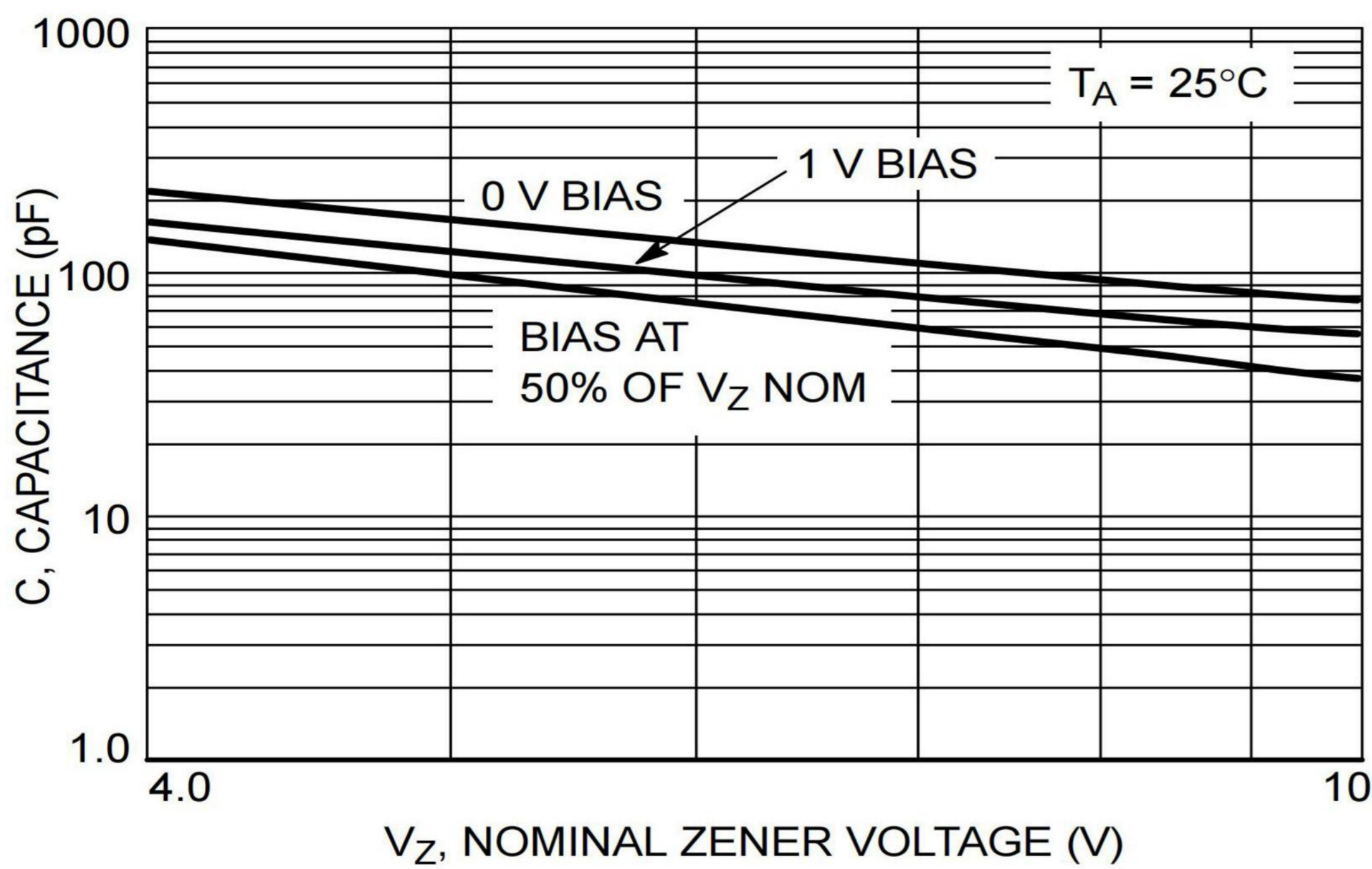
Figure 3. Typical Capacitance
