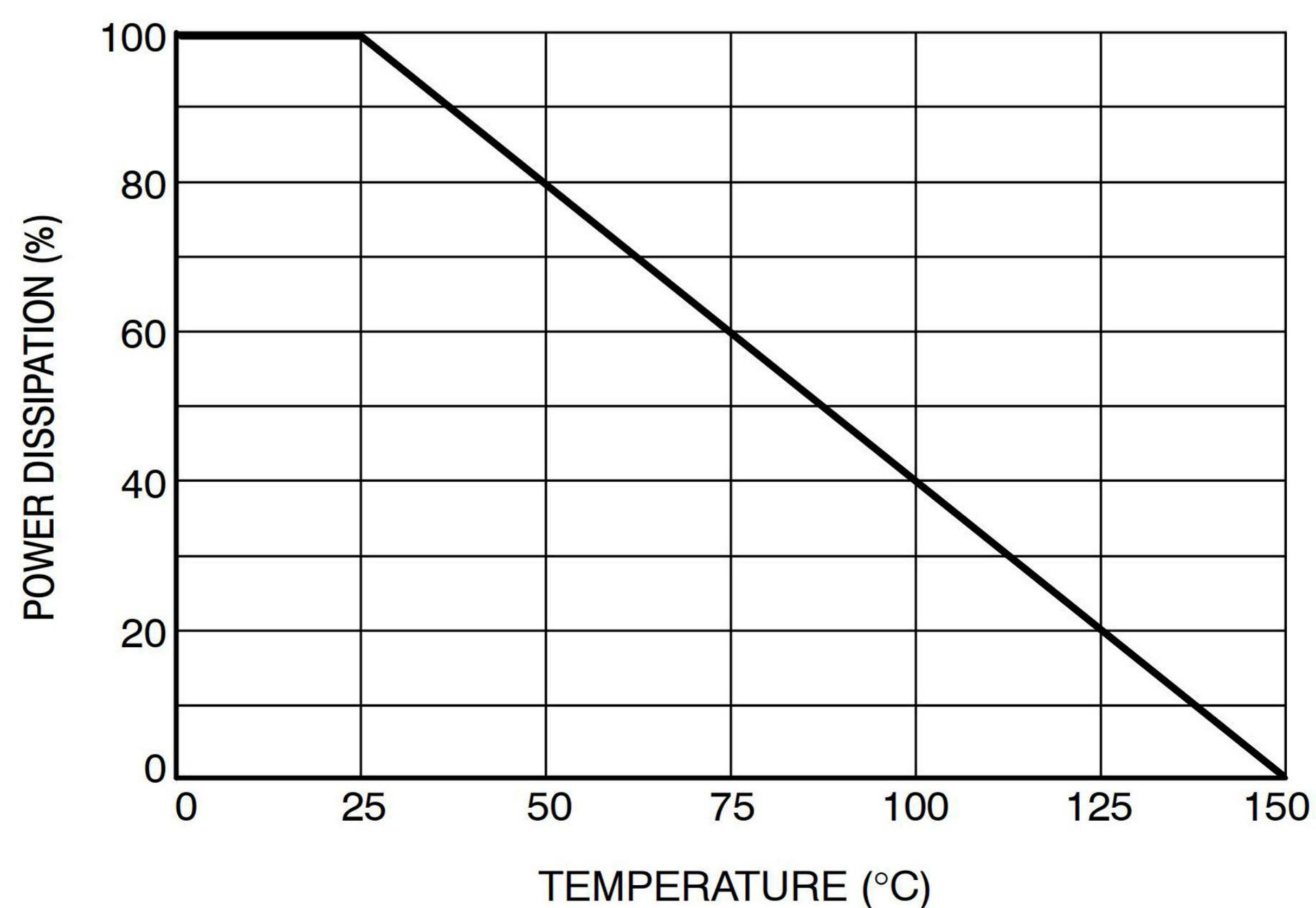
Figure 1. Steady State Power Derating
