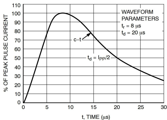
Figure 1. Pulse Waveform, 8/20 \mu\text{s}
