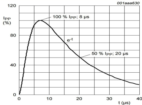
Fig. 1. 8/20 \mu s pulse waveform according to IEC 61000-4-5
