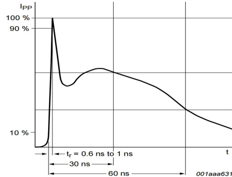
Fig. 2. ESD pulse waveform according to IEC 61000-4-2
