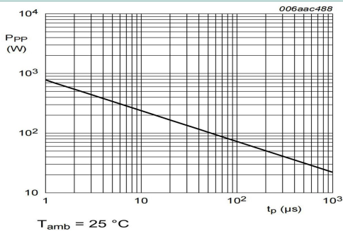
Fig. 3. Peak pulse power as a function of exponential pulse duration; typical values
