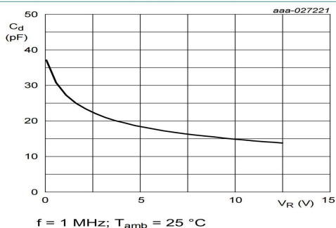
Fig. 5. Diode capacitance as a function of reverse voltage; typical values
