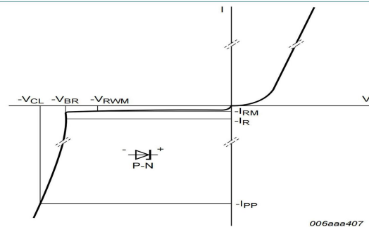
Fig. 6. V-I characteristics for a unidirectional ESD protection diode
