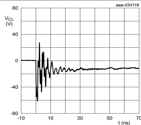
Fig. 6. Clamped -8 kV ESD pulse waveform (IEC 61000-4-2 network)
