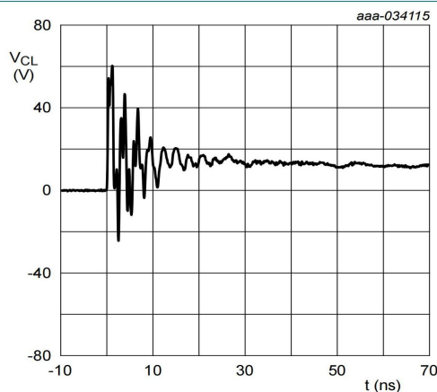
Fig. 5. Clamped +8 kV ESD pulse waveform (IEC 61000-4-2 network)
