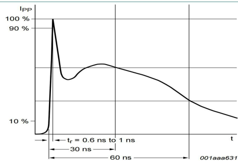
Fig. 2. ESD pulse waveform according to IEC 61000-4-2
