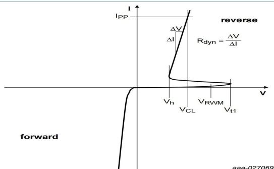
Fig. 3. Typical Transmission Line Pulse (TLP) characteristics for a unidirectional ESD protection device for data lines
