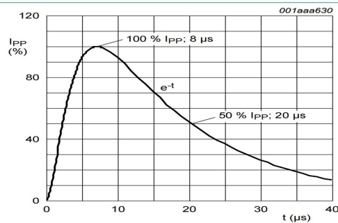
Fig. 1. 8/20 \mu s pulse waveform according to IEC 61000-4-5
