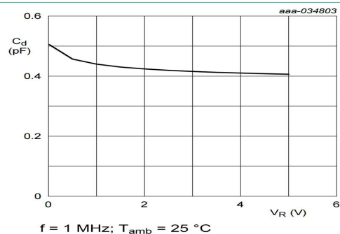
Fig. 4. Diode capacitance as a function of reverse voltage; typical values
