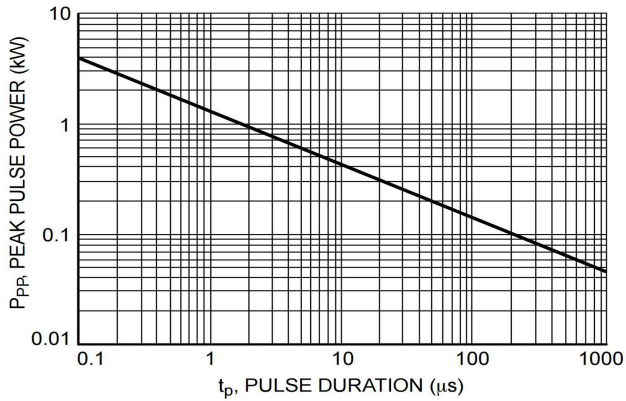
Figure 1. Non-Repetitive Peak Pulse Power versus Pulse Time
