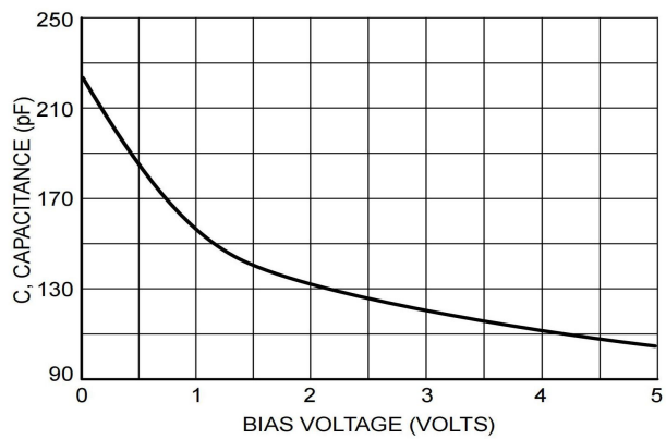
Figure 4. Typical Diode Capacitance (SM05)
