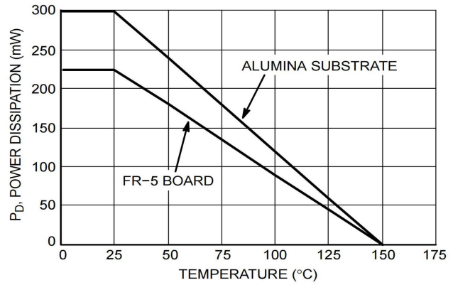
Figure 2. Steady State Power Derating Curve
