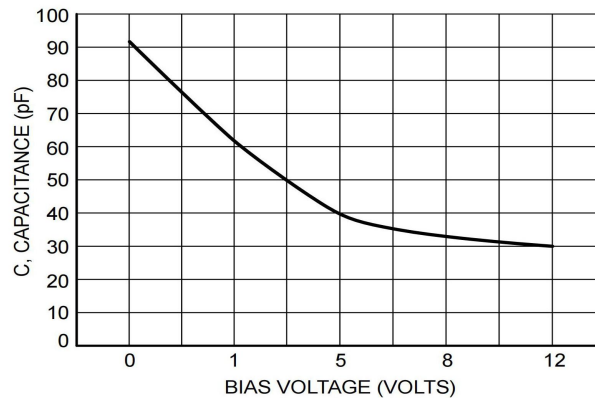
Figure 5. Typical Diode Capacitance (SM12)
