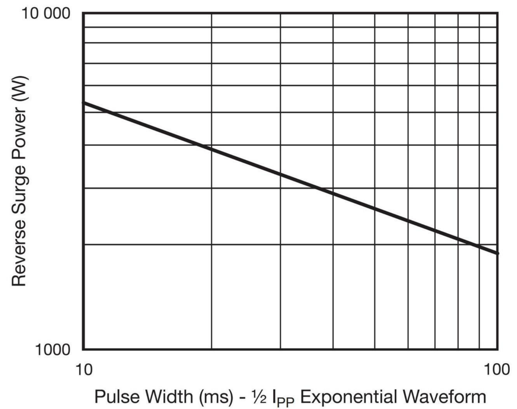
Fig. 4 - Reverse Power Capability
