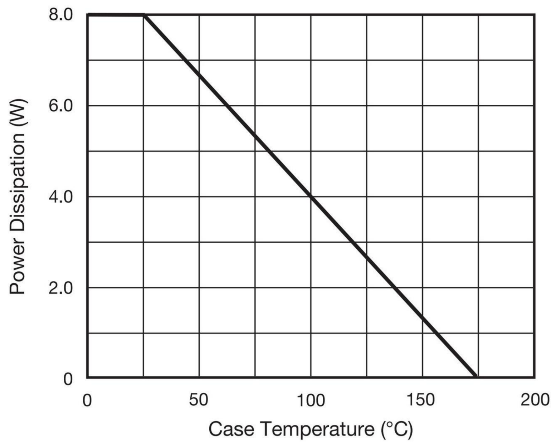
Fig. 1 - Power Derating Curve
