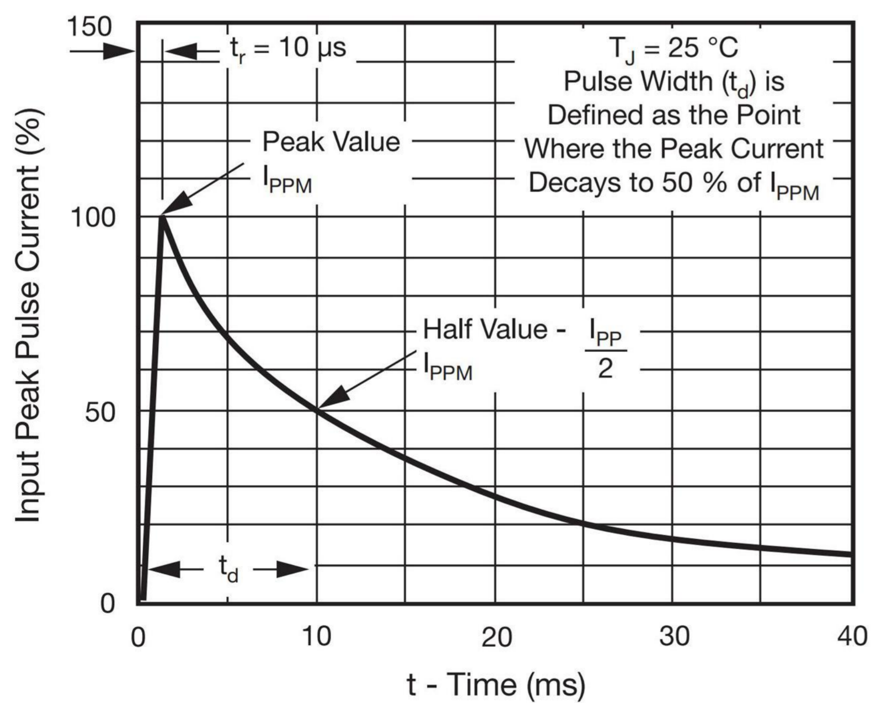
Fig. 3 - Pulse Waveform
