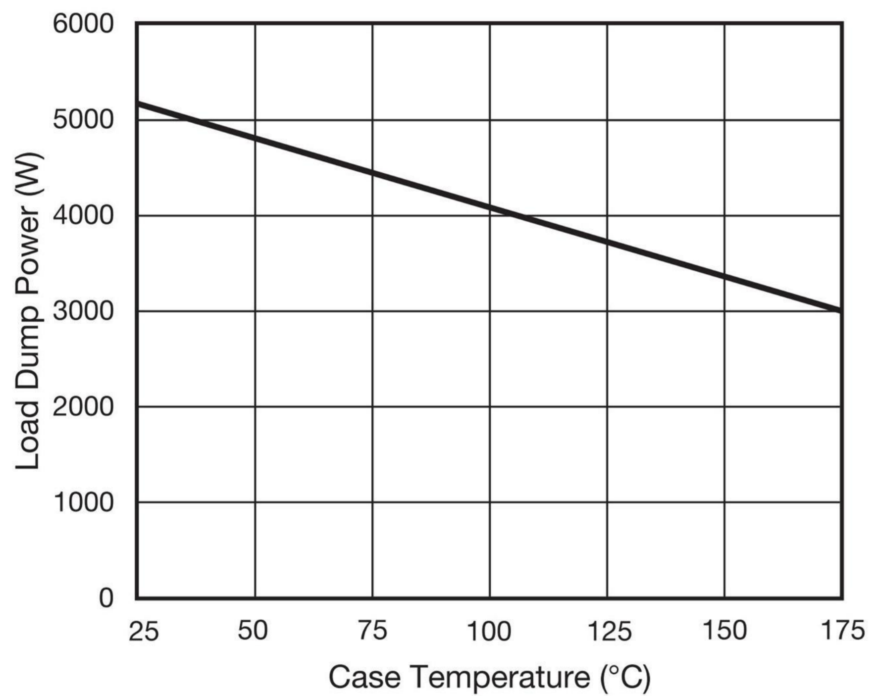
Fig. 2 - Load Dump Power Characteristics (10 ms Exponential Waveform)
