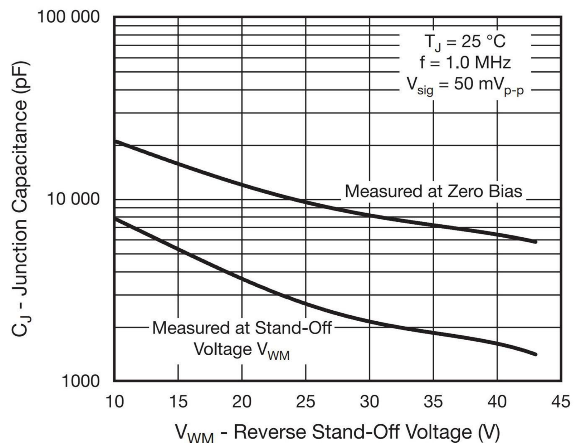
Fig. 6 - Typical Junction Capacitance
