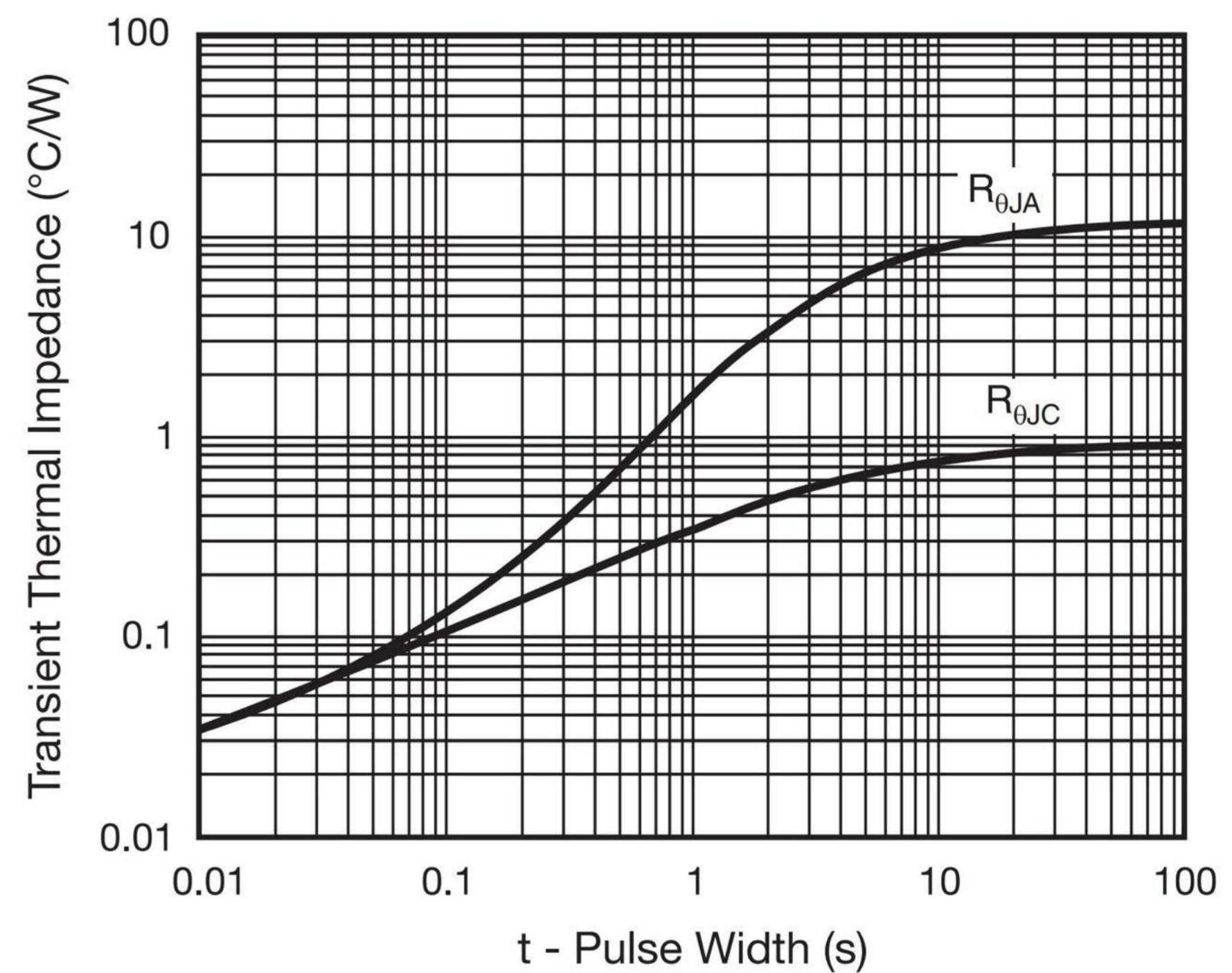
Fig. 5 - Typical Transient Thermal Impedance
