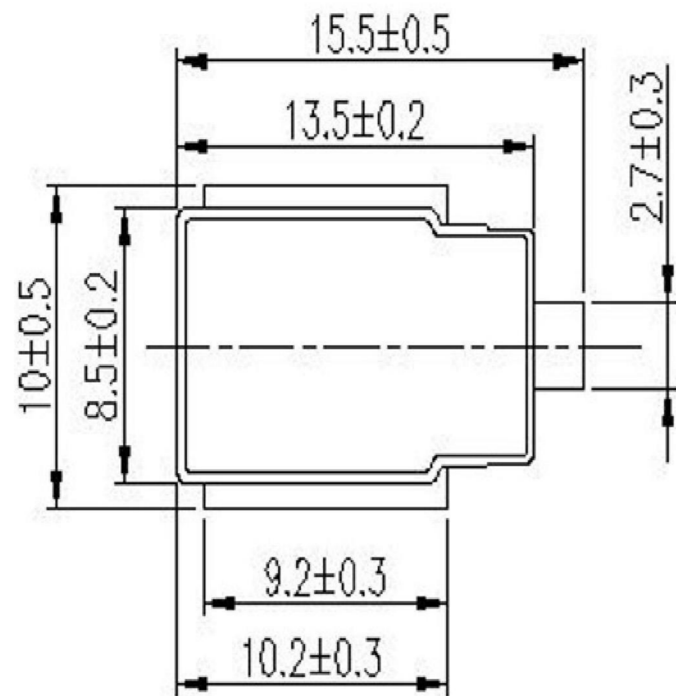
DO-218AB
