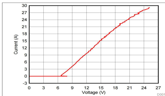
Figure 1. Positive TLP Curve
