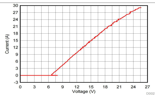
Figure 2. Negative TLP Curve
