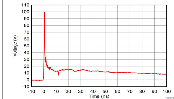
Figure 3. 8-kV IEC Waveform
