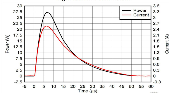
Figure 5. Surge Curve ( t_p = 8/20\mu\text{s} ), IO pin to GND
