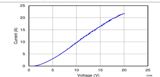
图 5-4. Negative TLP Plot IO to GND
