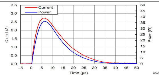
图 5-2. Surge Curve ( t_p = 8/20 \mu s , Pin IO to GND)
