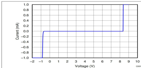
图 5-1. DC Voltage Sweep I-V Curve
