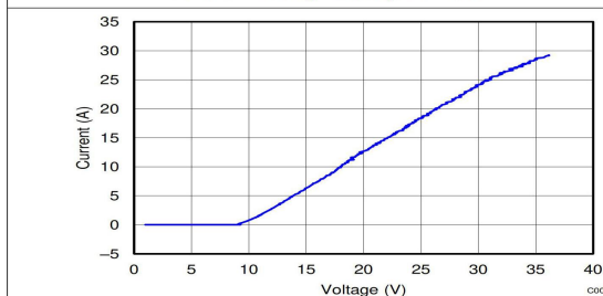
图 5-3. Positive TLP Plot IO to GND
