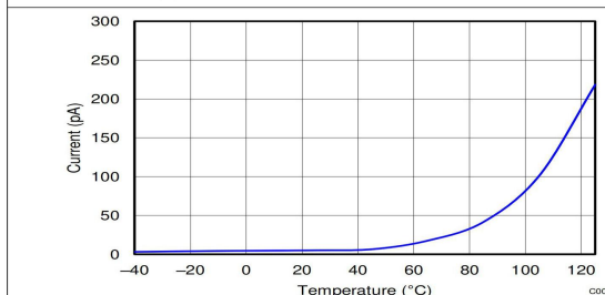
图 5-5. Leakage vs Temperature
