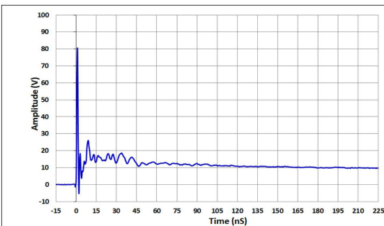
图 5-1. IEC 61000-4-2 Clamp Voltage +8 kV Contact ESD
