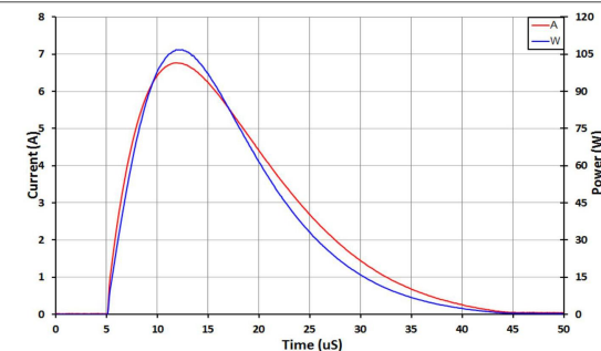
图 5-6. Positive Surge Waveform 8 to 20 \mu s
