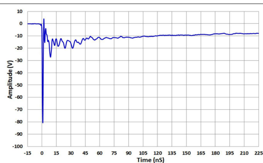
图 5-2. IEC 61000-4-2 Clamp Voltage -8-kV Contact ESD
